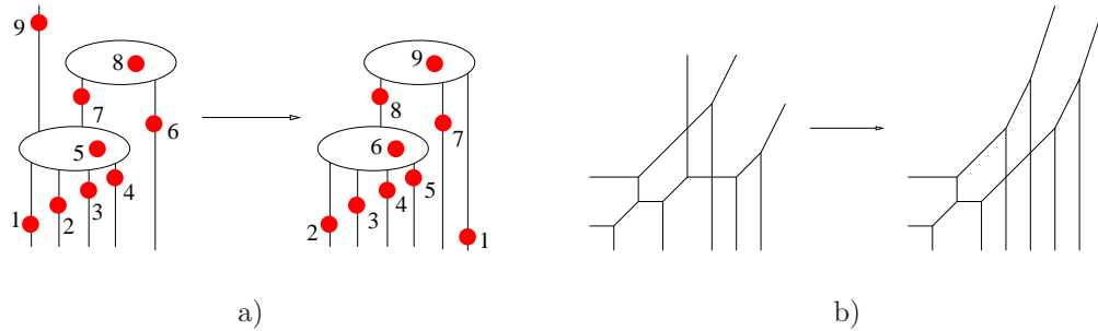
FIGURE 17. From \mathbb{F}_n to \mathbb{F}_{n+1}
