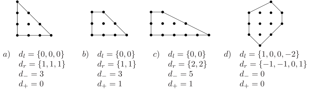
FIGURE 1. Examples of h -transverse polygons
