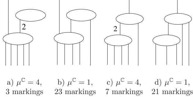
FIGURE 4. Floor diagrams of genus 0 and Newton polygon depicted in Figure 1c
