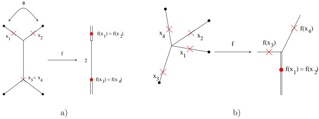
FIGURE 8. Real tropical curves
