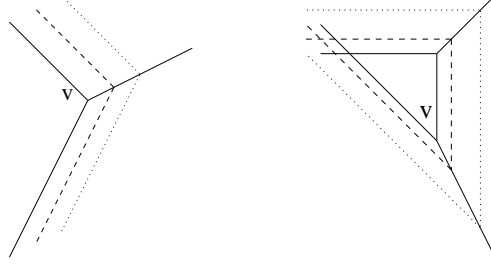
FIGURE 11. 1-parameter family of tropical curves
