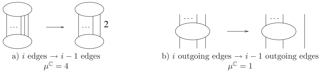
FIGURE 14. Decrease by 1 the genus of the floor diagram of maximal genus
