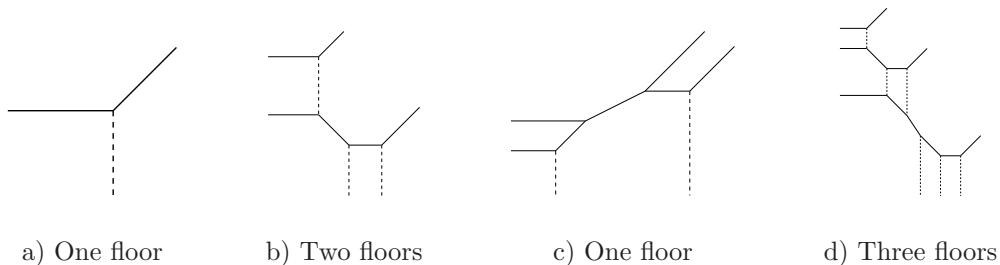
FIGURE 10. Floors of tropical curves
