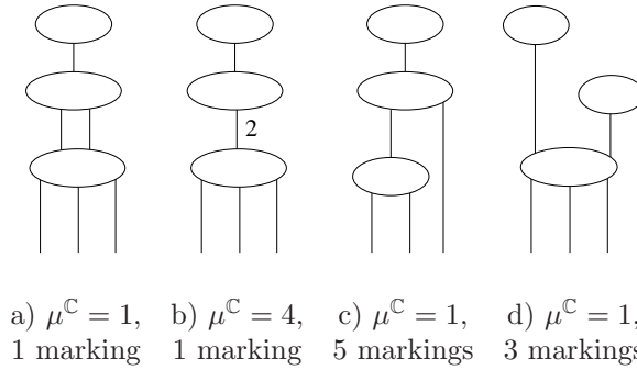
FIGURE 3. Floor diagrams of genus 1 and 0, and Newton polygon \Delta_3
