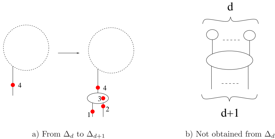
FIGURE 15. The numbers W(\Delta_d, 0) are increasing
